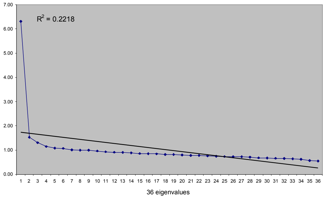
Figure 1: scree plot for data set E (36 eigenvalues).
